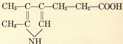
Isophonopyrrol carboxylic acid β-propionic acid-α', β'-dimethyl pyrrol
